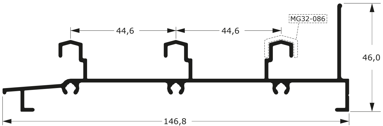
MG32-084 1,470 Kg/m
