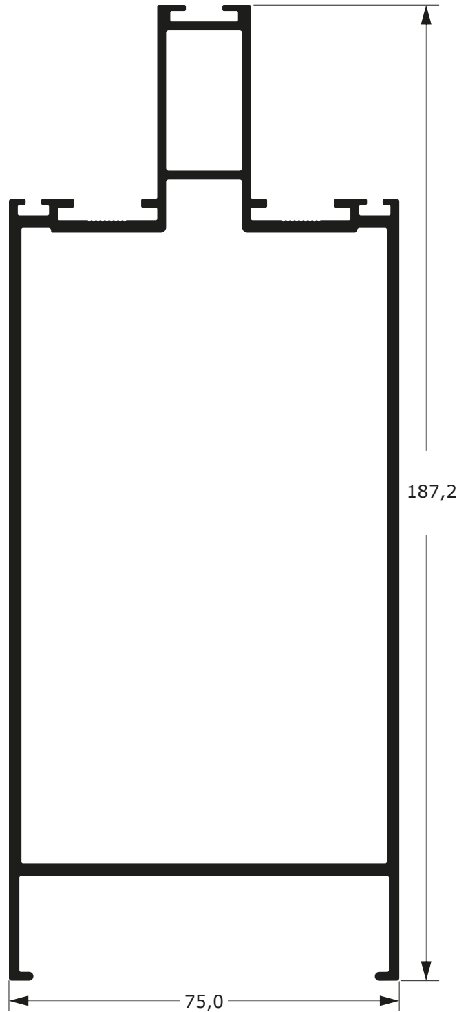
FC-233 3,392 Kg/m
