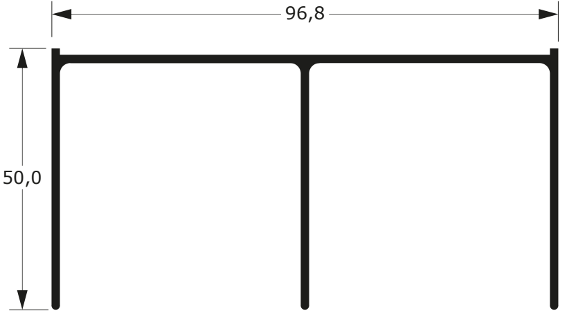
E-363 1,051 Kg/m
