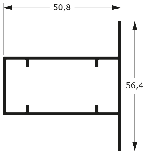
78-2427C 0,673 Kg/m
