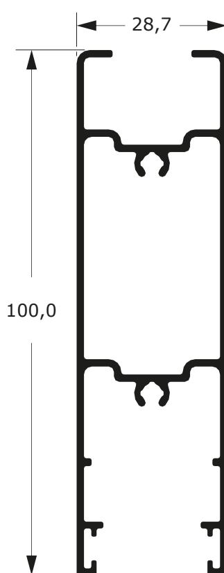
MG32-105 1,180 Kg/m
