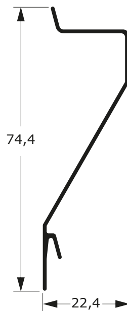
Z-203 Furada: Z-203F 0,291 Kg/m
