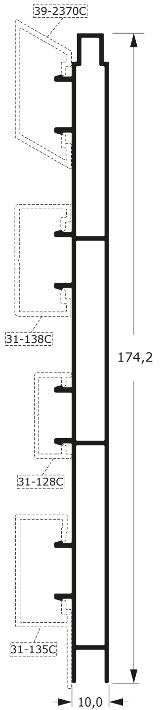
79-183D 1,395 Kg/m
