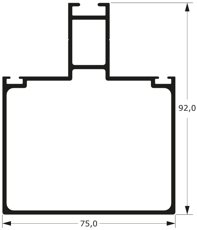
FC-075 1,750 Kg/m
